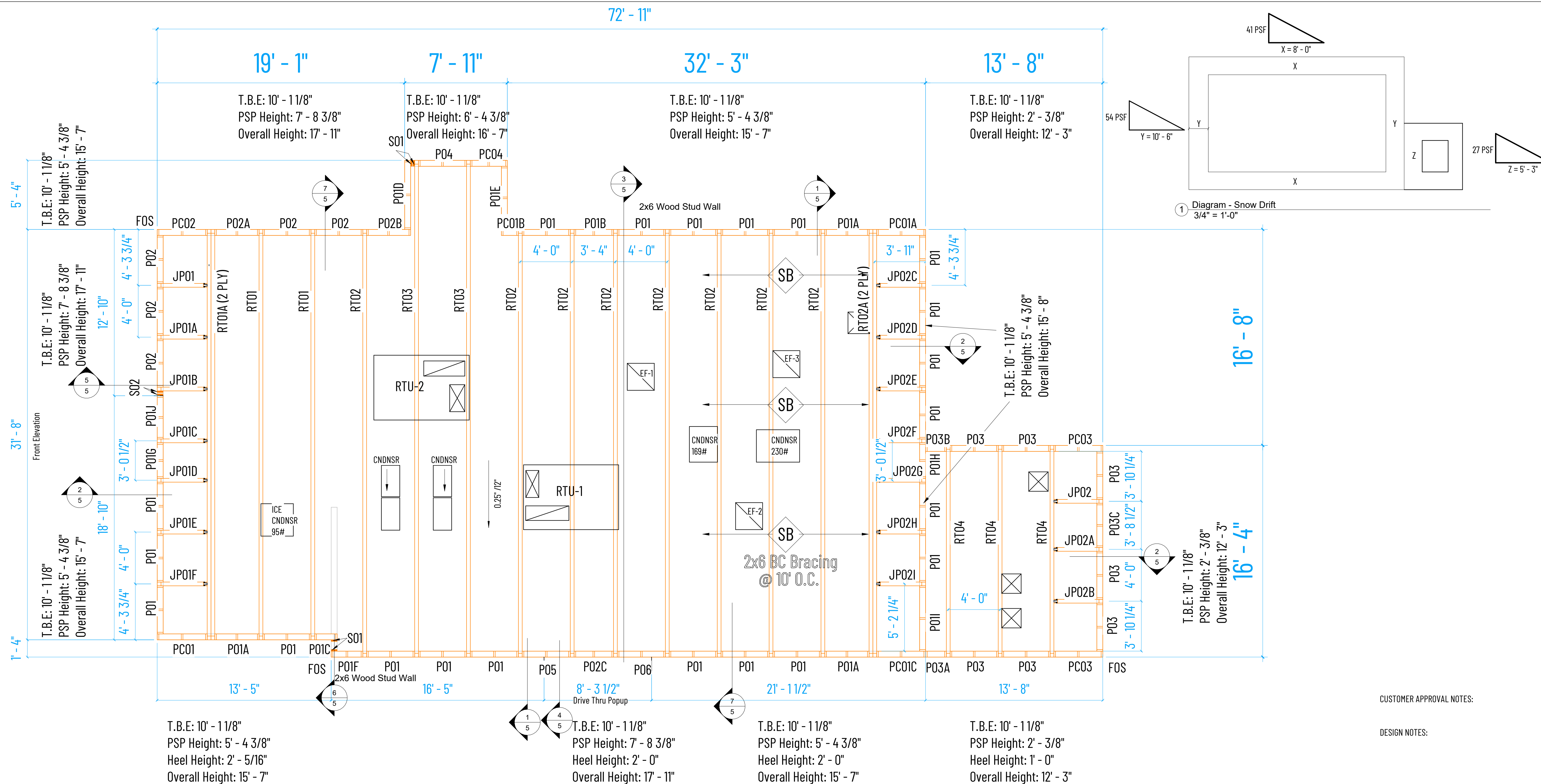
Truss Layout 1/4" = 1'-0"
